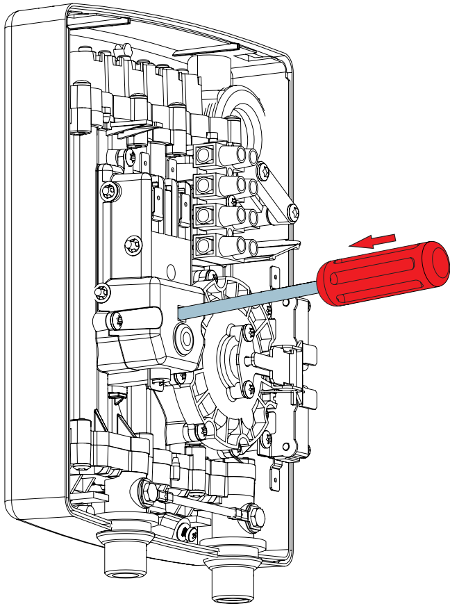
Pic. 5. Switching on the pressure fuse
